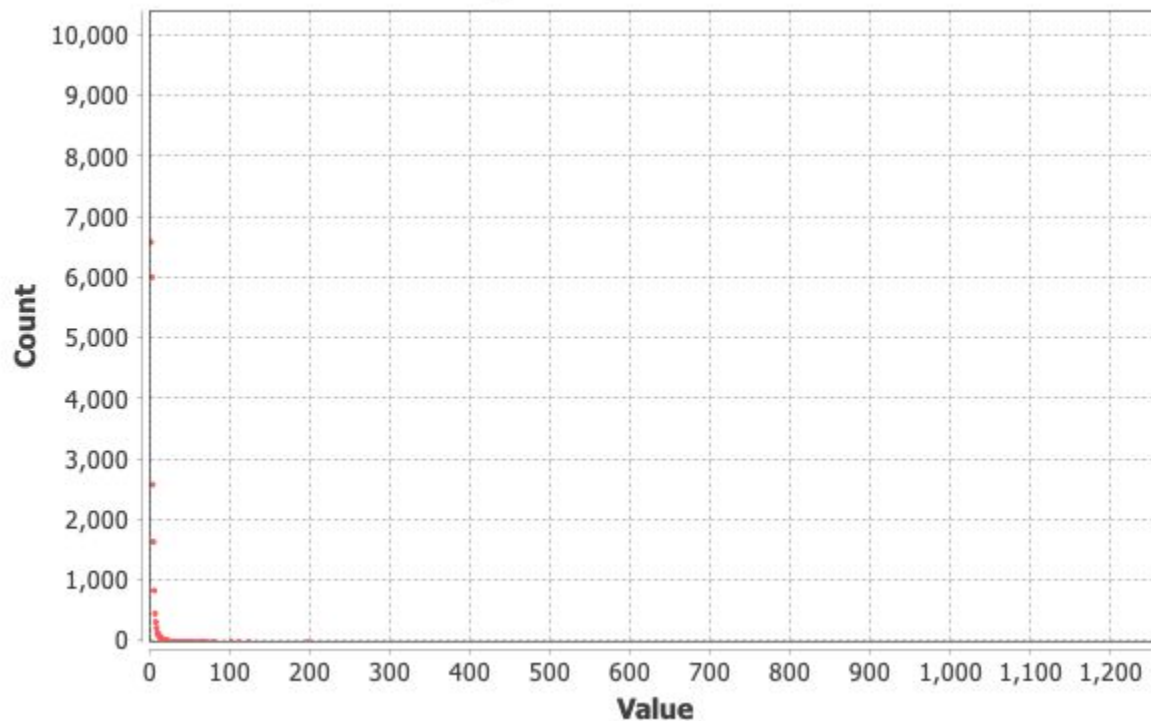
Out-Degree Distribution
