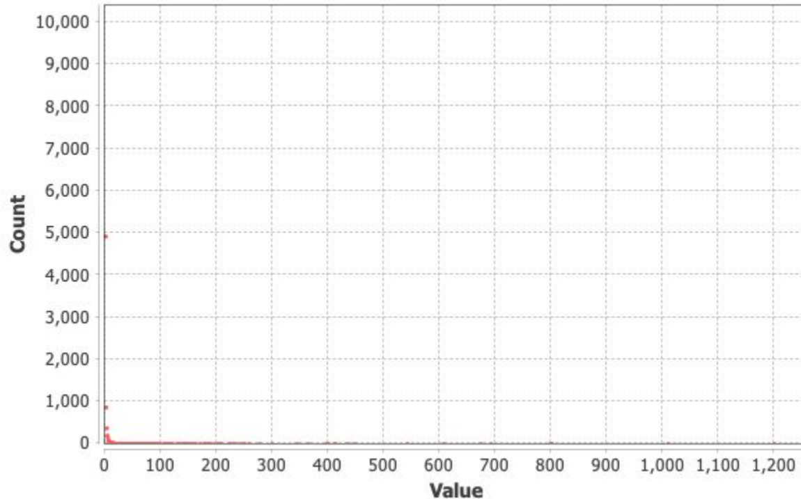
In-Degree Distribution
