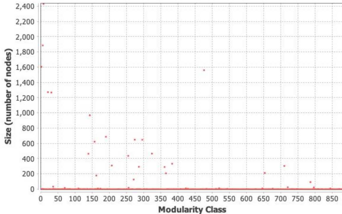
Size Distribution
