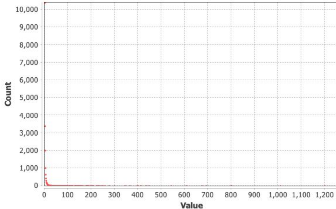
Degree Distribution
